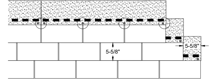
Figure 6 - 3-Tab, 4-Nail Fastening Pattern
