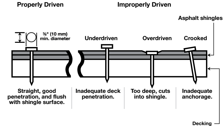
Figure 5 - Nailing Instructions
