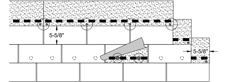
Figure 7 - Hand-Sealing 3-Tab Shingles
