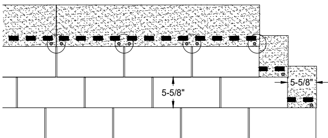
Figure 8 - 3-Tab, 6-Nail Fastening Pattern
