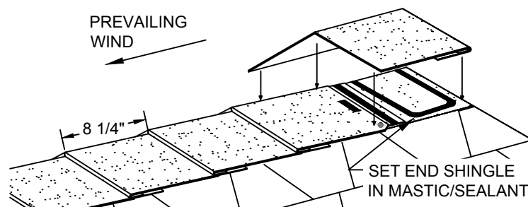
Figure 26 - Optional Positioning and Fastening of the EZ-Ridge™ End Cap
