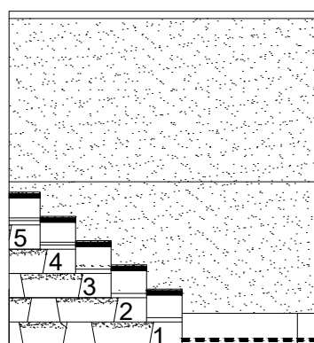
Figure 10 - Laminate Shingle Layout Pattern
