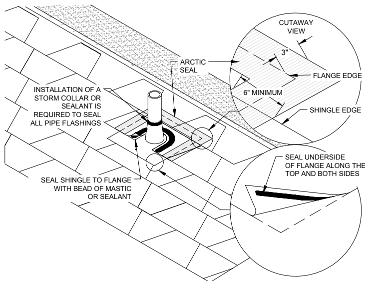
Figure 14 - Vent Pipe Flashing Application
