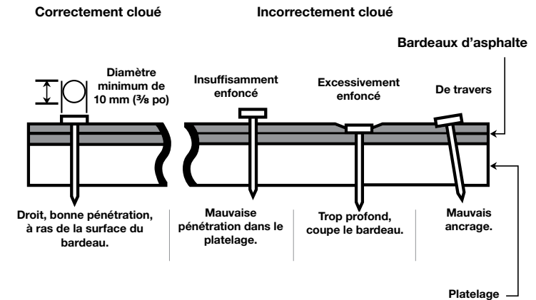
Figure 5 – Instructions de cloutage
