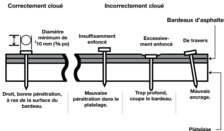
Figure 5 – Instructions de clouage
