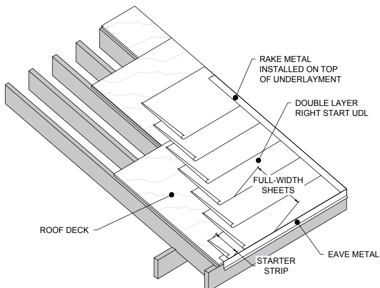
Figure 2 - Application of Right Start™ UDL on Roof Slopes 2:12 Up to 4:12 (Non-Ice Dam Regions)
