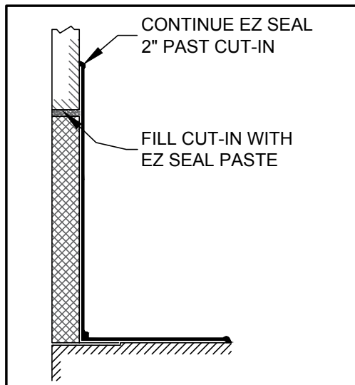
OPTION: COVER AND FILL CUT-IN
