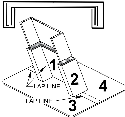
EZ SEAL FLEECE CUT TO MATCH SUBSTRATE/PENETRATION ANGLE
