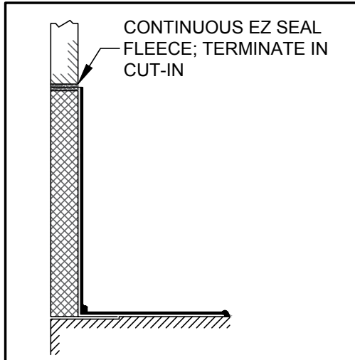
OPTION: CONTINUOUS EZ SEAL INTO CUT-IN
